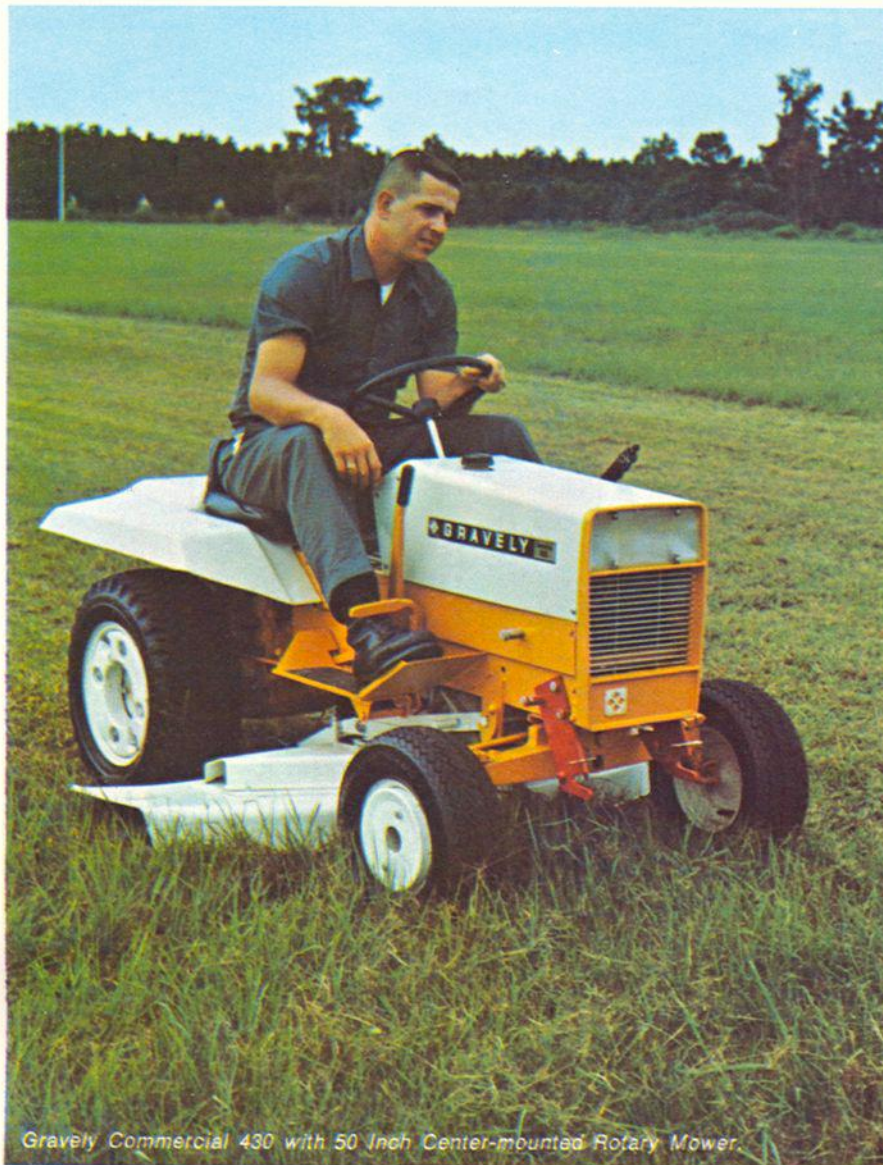
Commercial 430 with 50 Inch Commercial Mower. Optional Wheel Weights.
